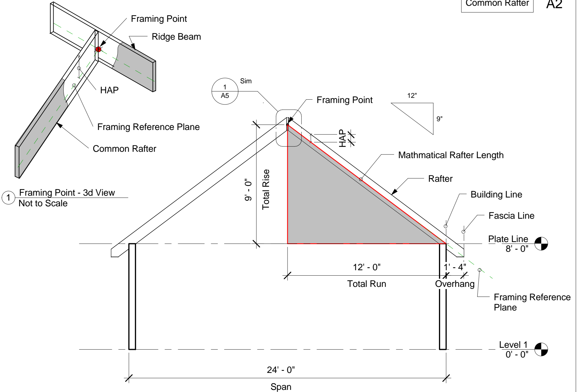
Ⓐ Section A 1/4" = 1'-0"
