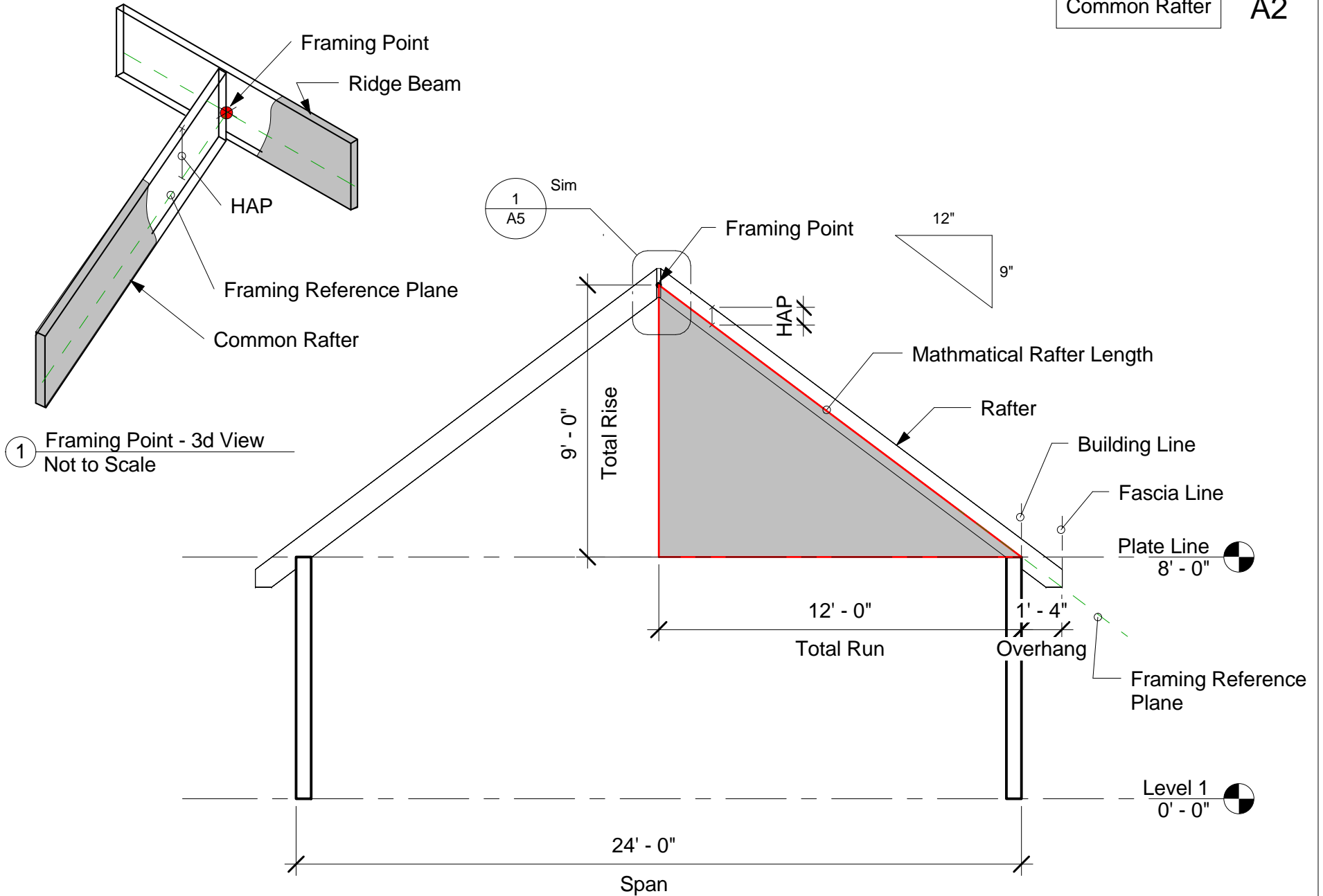
A Section A 1/4" = 1'-0"
